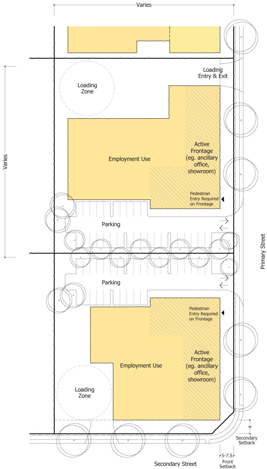
Employment Building Typology 6 Individual Parking and Seperate Loading
