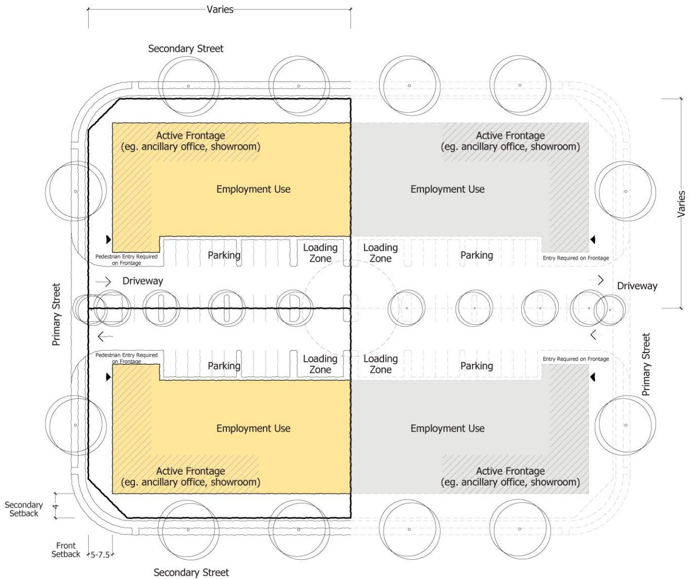
Employment Building Typology 1 Shared Parking and Loading Access
